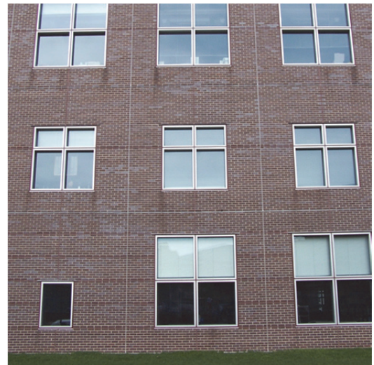
Figure 11: Placement of movement joints creates wall symmetry.
